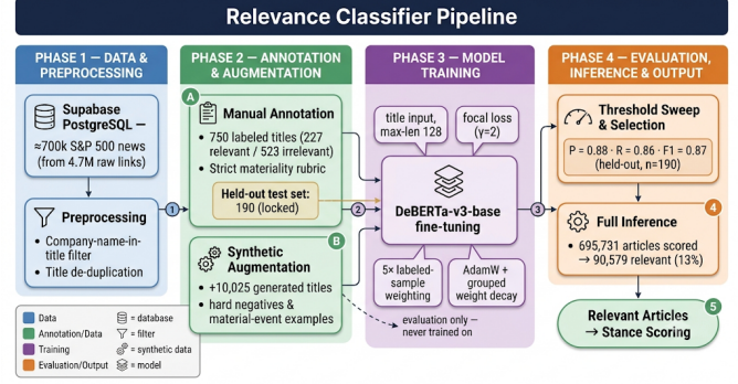
Fig. 2. Relevance classifier pipeline: raw S&P 500 news titles, preprocessing, manual annotation and synthetic augmentation, DeBERTa-v3 fine-tuning, threshold selection on a held-out test set, and full-corpus inference.
