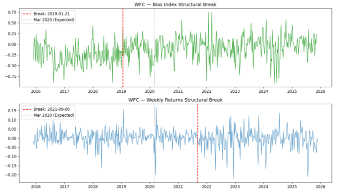
Fig. 7. Bai-Perron structural breaks for Wells Fargo (WFC), one of two firms with a cointegrating bias-return relation; its return-to-bias feedback emerges only post-break.
